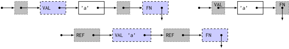
Fig. 7. Three different uniform representations of a value of type \text{char stream} . The top-left representation is how the value is represented in \text{MLKit}^\dagger (without unboxing) whereas the top-right representation is how the value is represented unboxed in \text{MLKit} using high-bit pointer tagging. The representation below is how the value is traditionally represented in ML implementations such as \text{MosML} , \text{OCaml} , and \text{SML/NJ} . Gray (and dotted) boxes represent \text{ref} cells, the light-blue (and dashed) rectangular boxes represent boxed constructed values, and the white rectangular boxes represent pairs.
