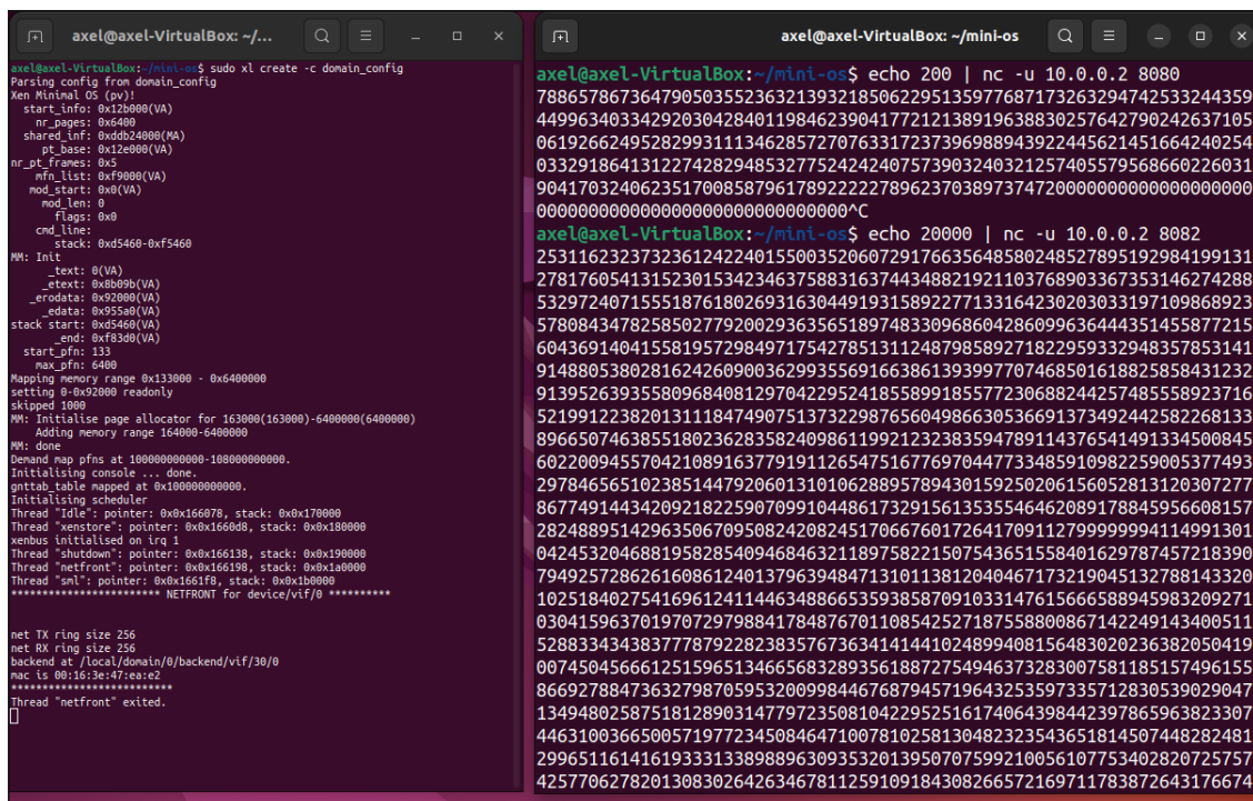
Figure A.1: The facfib service running on Xen. Here factorial 200 is requested on port 8080, and then fibonnaci for 20000 is requested on port 8082.
