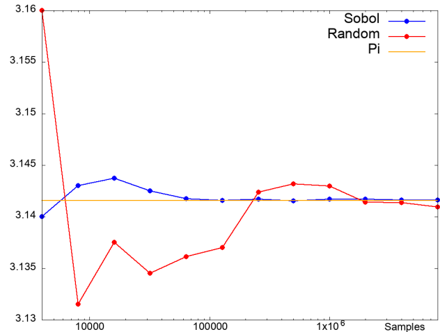
Figure 11. Convergence towards \pi using Sobol sequences and pseudo-random numbers.
