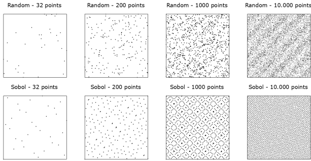
Figure 7. Points spanning the unit-square for a progressive number of points, using pseudo-random numbers (top row) and Sobol sequences (bottom row).
