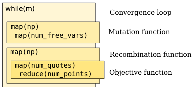
Figure 12. Loop Structure of the Heston Calibration benchmark. The coloured boxes and their labels indicate the logical nesting of the code, and in parentheses the number of iterations. All loops are parallel, except for the outer convergence loop. One loop is a reduce , while the others are maps .
